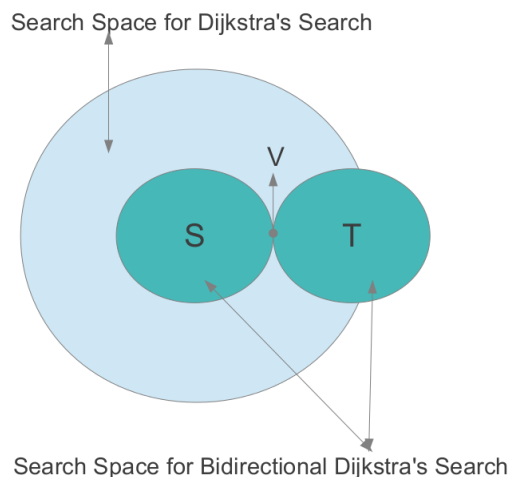
Figure 4.2: Search Space: Dijkstra's search vs. Bidirectional Search
