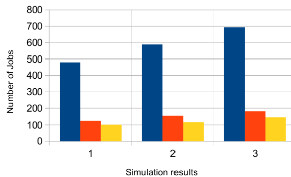
Figure 3.1: Simulation with \alpha = 0.5 and two worker threads
